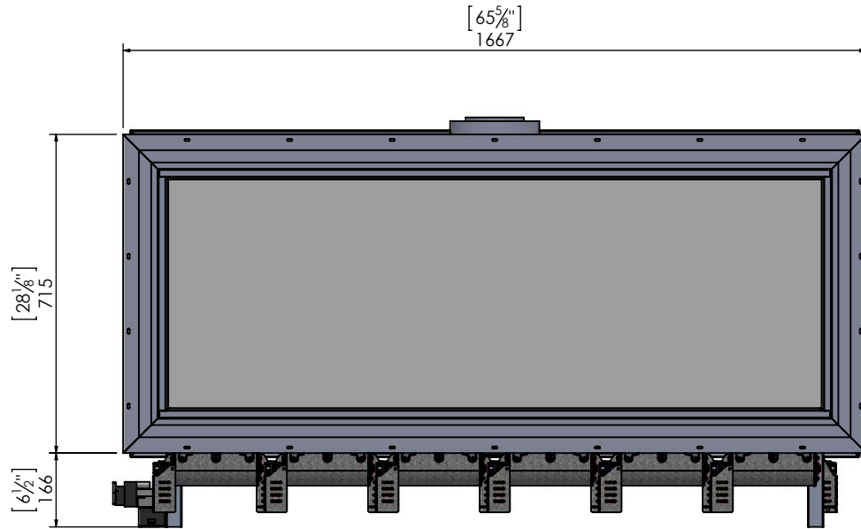
OUTSIDE VIEW
