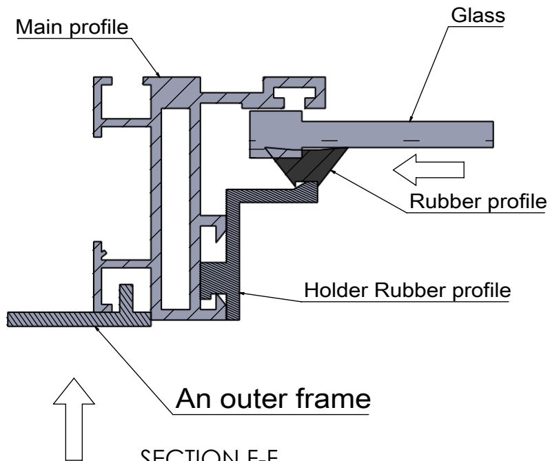
SECTION F-F SCALE 1 : 1
